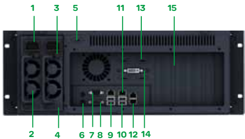
Performance Magelis机架式电脑后视图(冗余电源)
