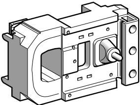
LC1FK●●●
