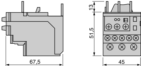
LR97D●●●●
